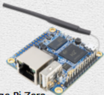
Orange Pi Zero
