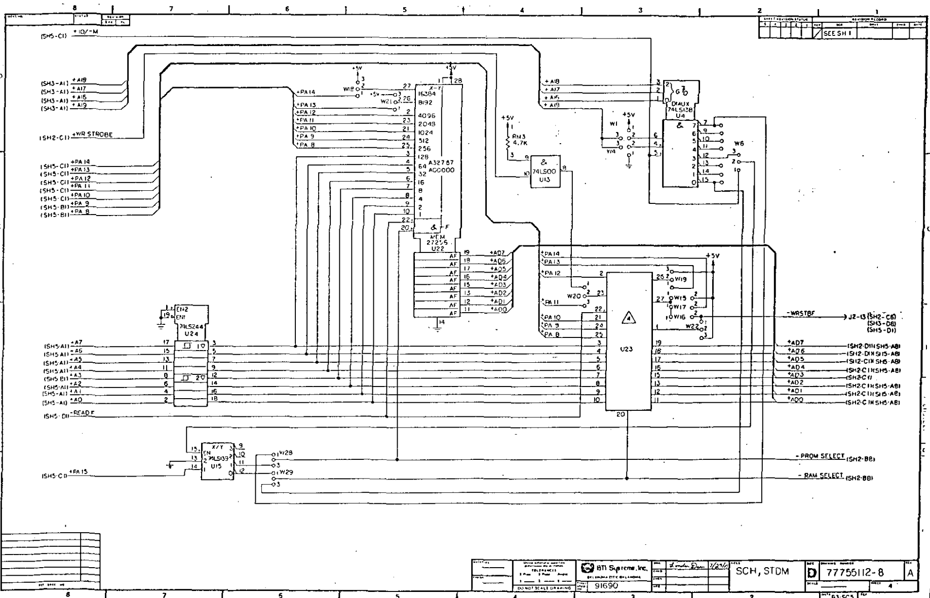
Figure 7.2-27 STD M PWA (6 OF 7)
