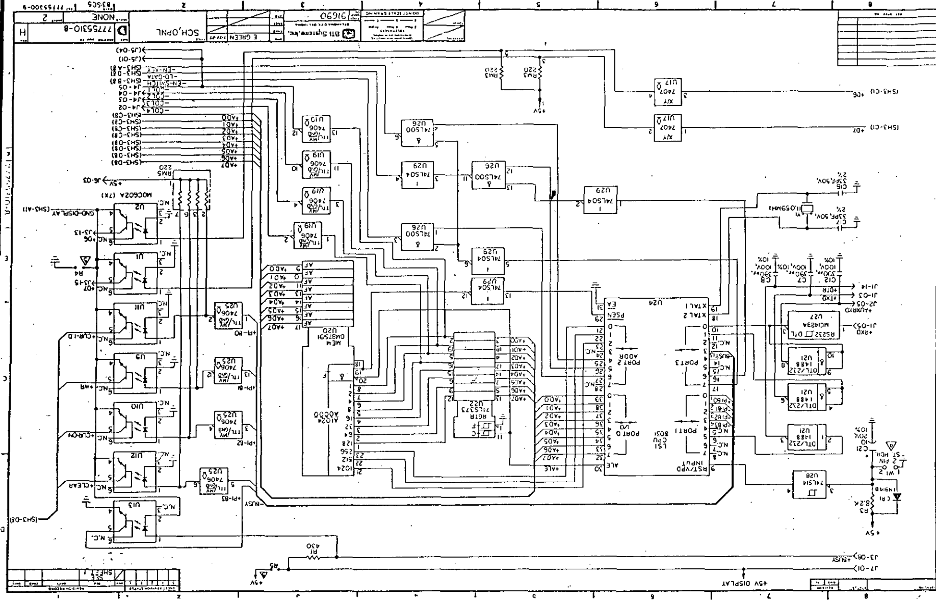
Figure 7.2-18 OPNL PWA (3 OF 4)
