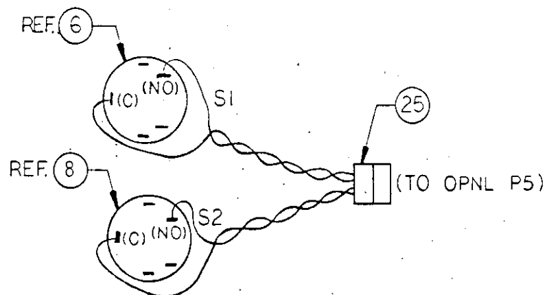
VIEW A
