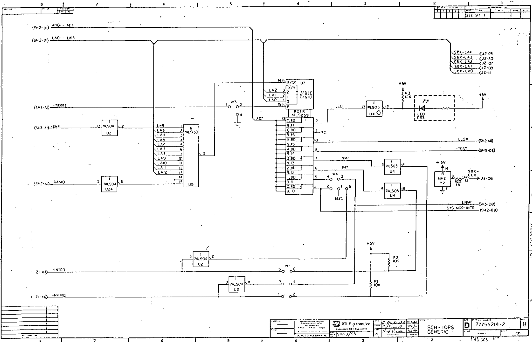
Figure 7-2-8 IEEE PWA (6 OF 6)
