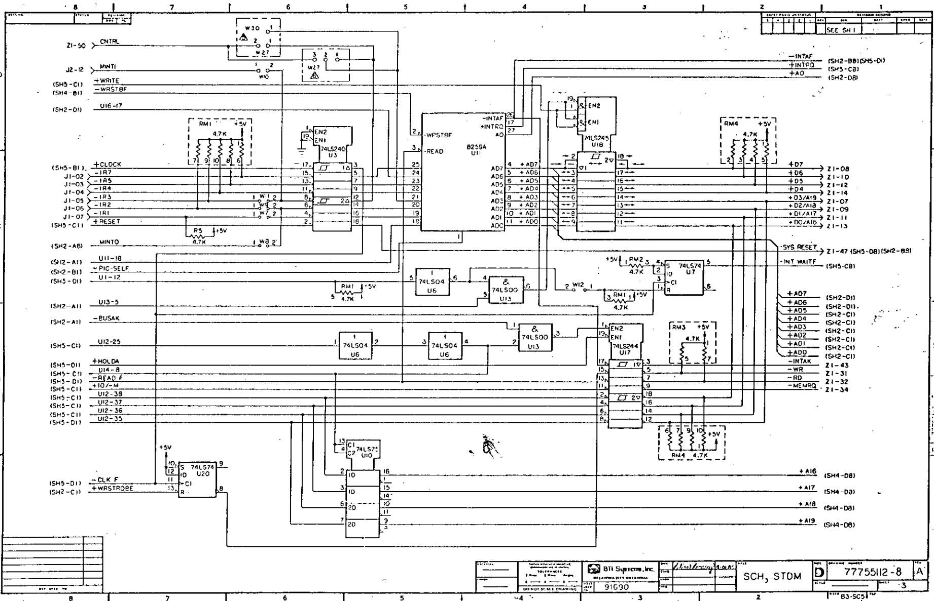
Figure 7.2-27 STD M PWA (5 OF 7)
