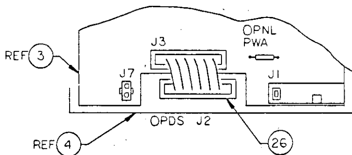
VIEW B
