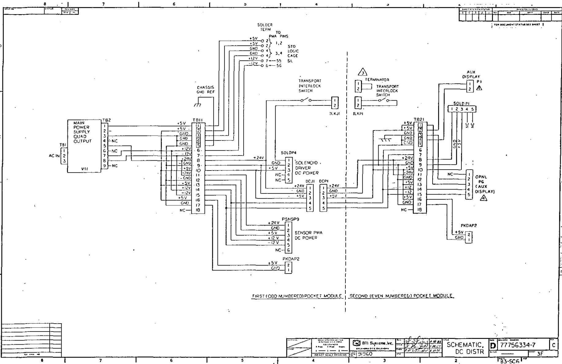
Figure 7.3-2 DC Power Distribution (3 OF 3)
