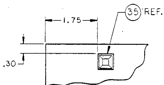
VIEW C
