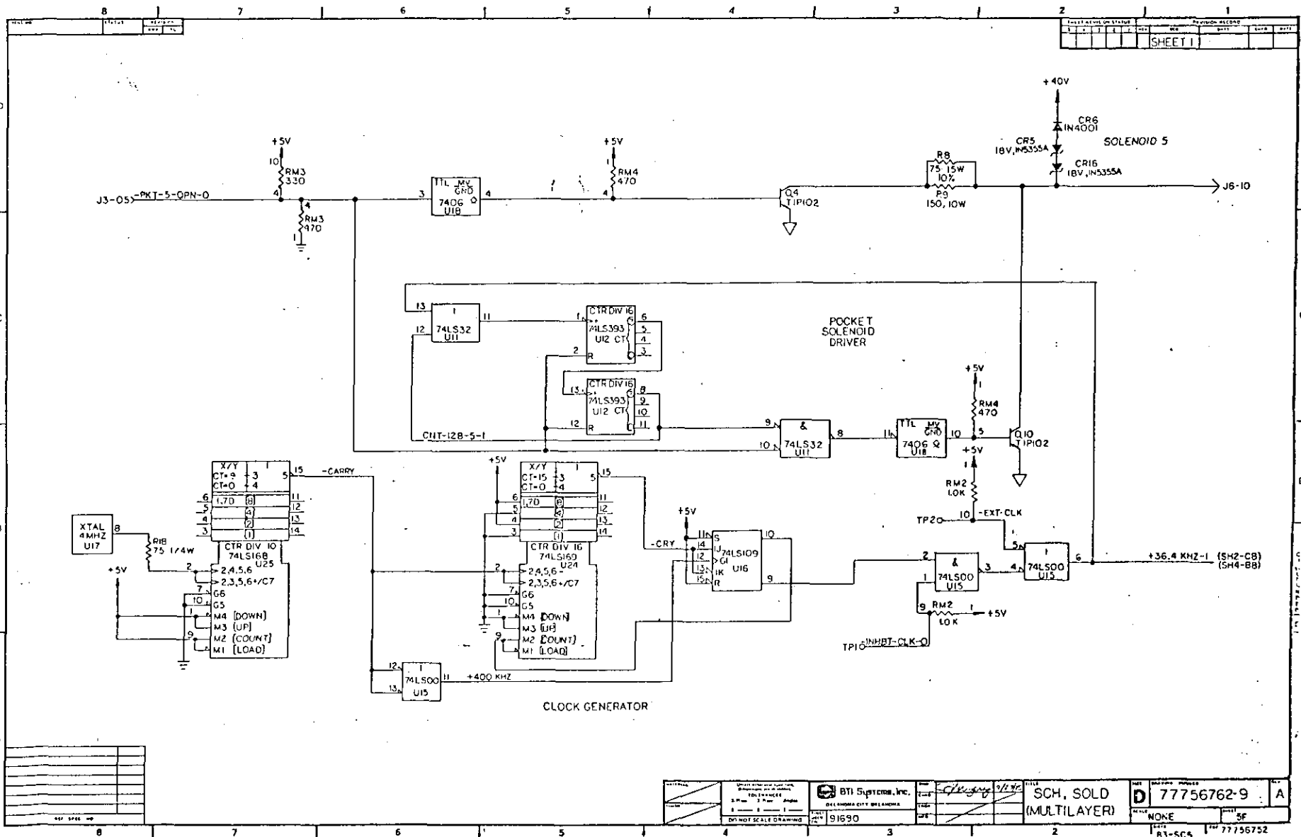
Figure 7.2-26 SOLD PWA (6 OF 6)
