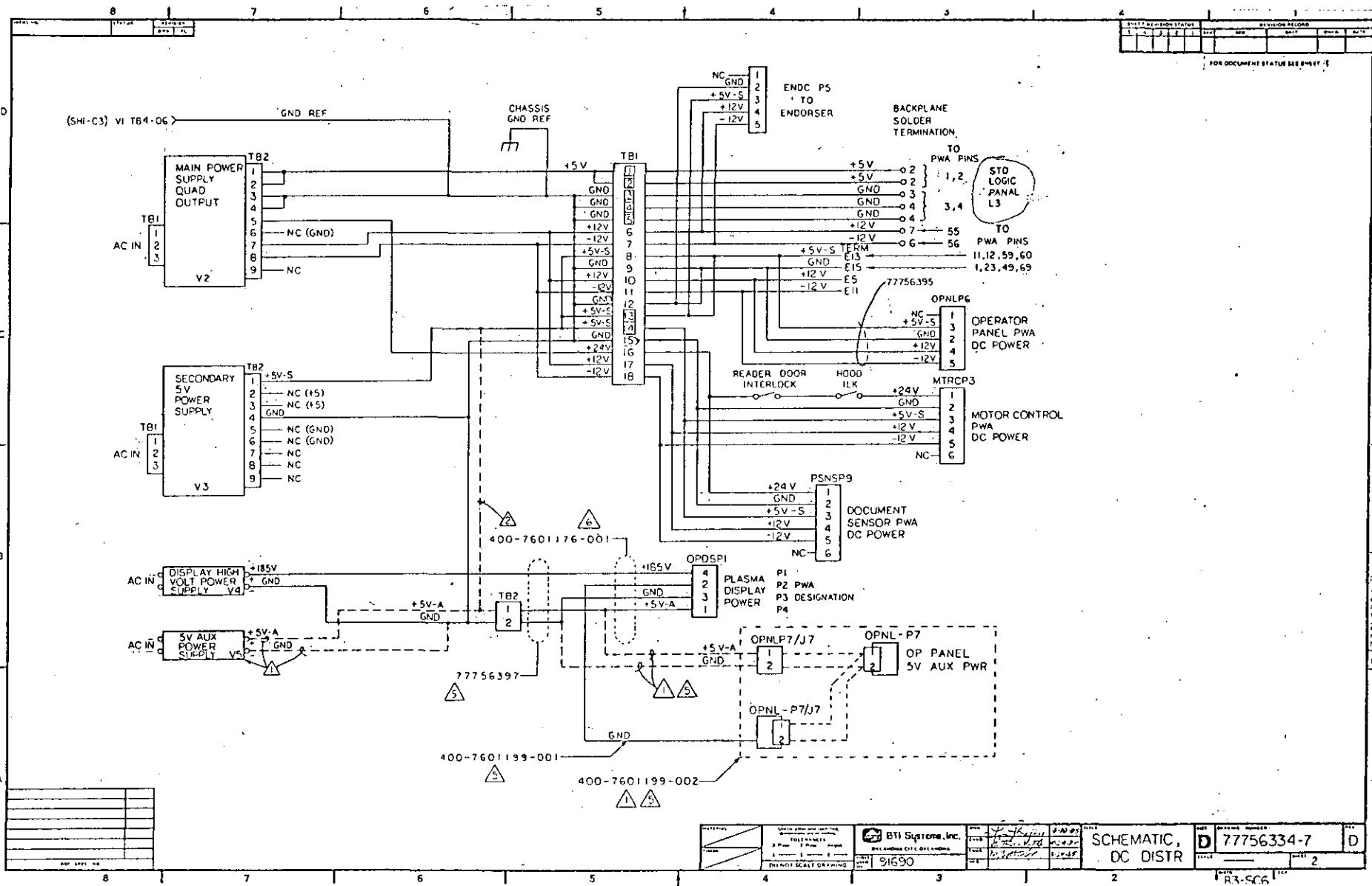
Figure 7.3-2 DC Power Distribution (2 OF 3)
